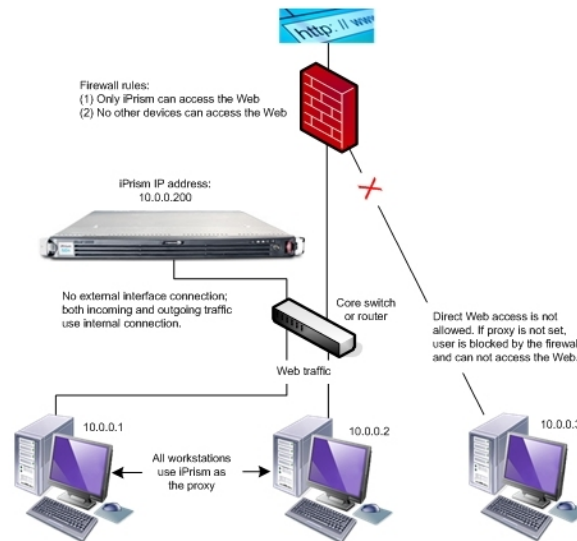
Figure 2. Deploying iPrism in Proxy Mode
